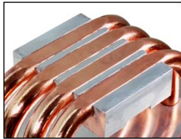
4 heatpipes and H.D.T. Core
