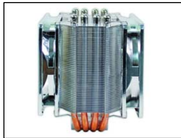
Two 12025 Fans
